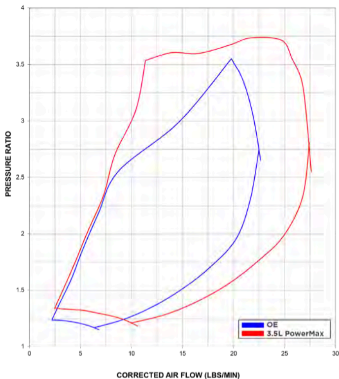
Compressor map comparison OE vs Garrett
